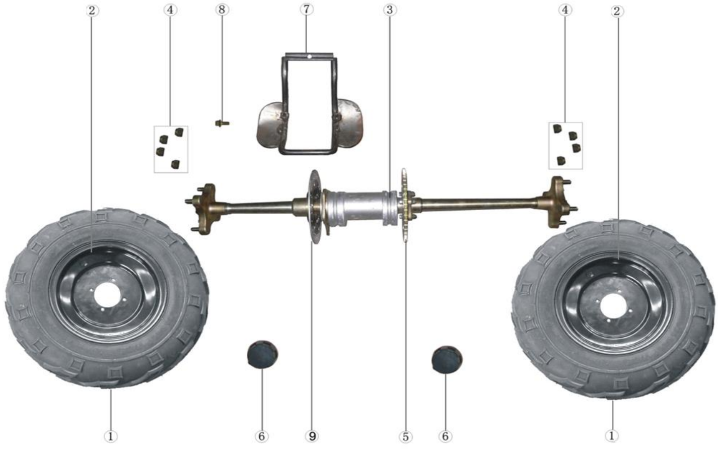
REAR WHEEL ASSEMBLY (4)
