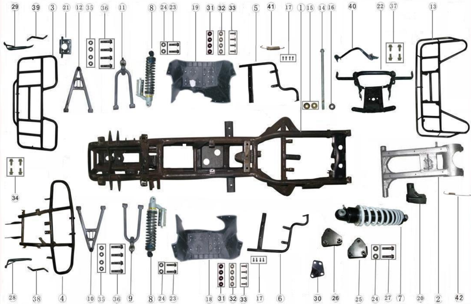
FRAME ASSEMBLY (1)
